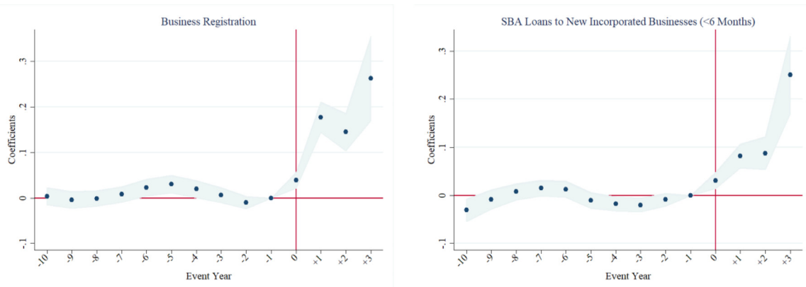
Fig. 2. Difference-in-Difference Estimators.
